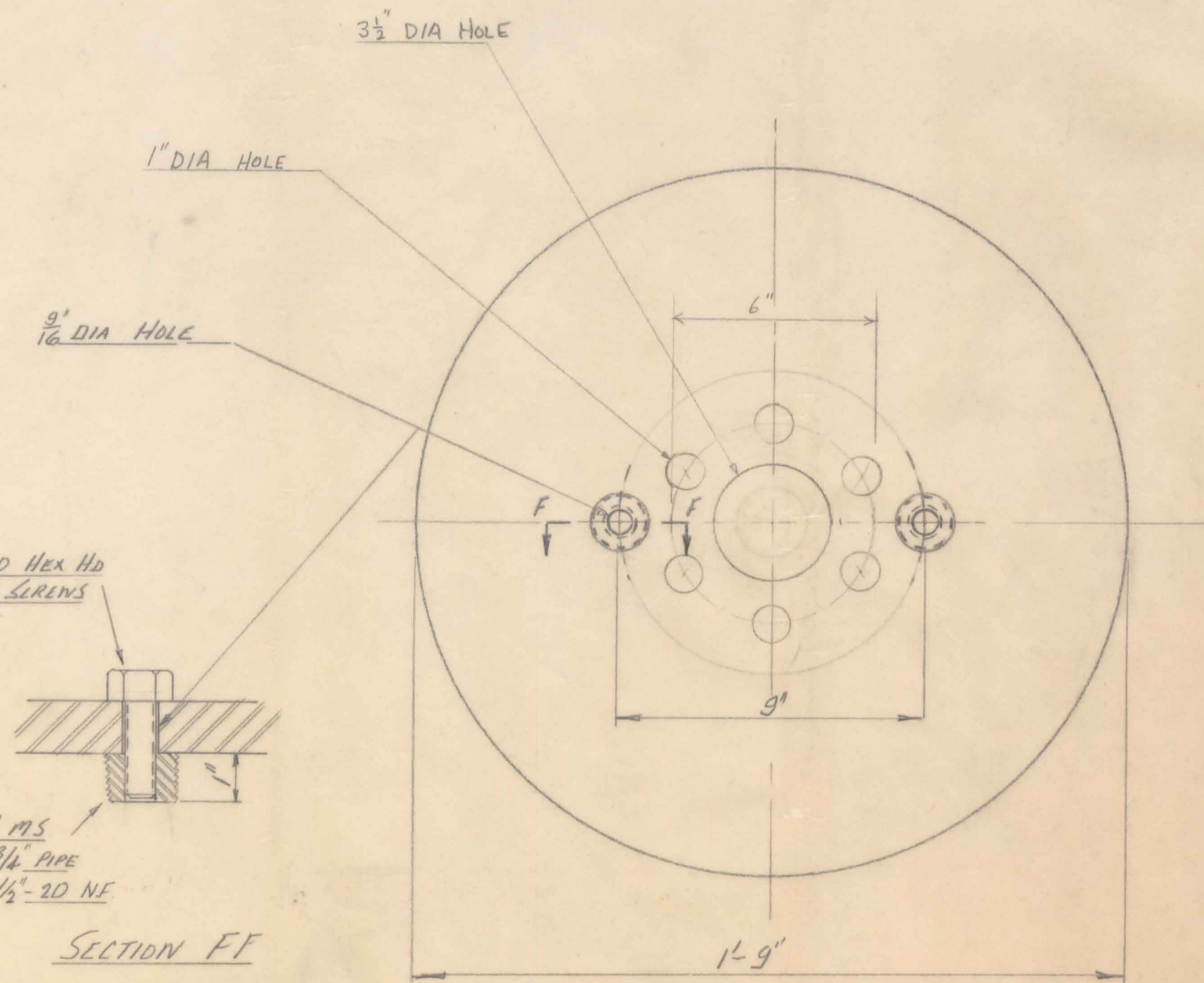
TOP PLATE 1 PER UNIT (TO BE WELDED IN ASSEMBLY AS PER DETAIL E) MAT 3/4" M.S.
