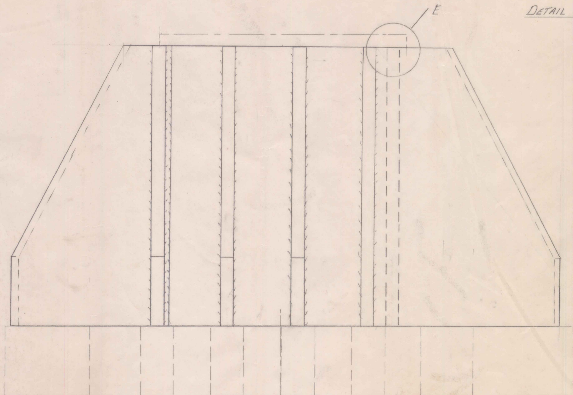
STEEL RING & GUSSET ASSEMBLY (ALL WELDED CONSTRUCTION)
